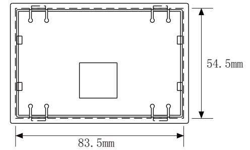
钣金安装开孔尺寸：83.5mm*54.5mm
